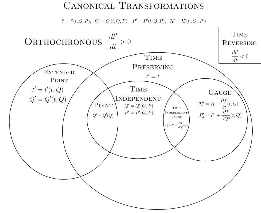
Figure 1.2: Some of the different classes of Canonical Transformations. One should note this diagram does not reflect the relative size of each set; the regions are not drawn “to scale”. The hierarchy of largest to smallest sets of transformations is: Canonical > Orthochronous = Time Reversing > Time-Preserving Canonical > Time Independent > Extended Point > Point > Gauge > Time Independent Gauge.
