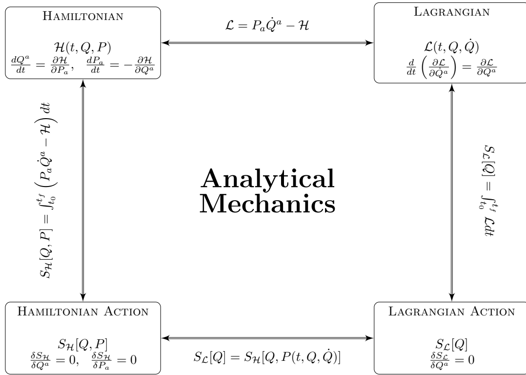
Figure 1.1: The core objects of Analytical Mechanics (and Physics by extension). If there is anything in this book you must know before you put it down, it is this chart.
