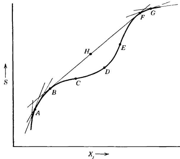
Figure 5.1: Figure taken from [13]. The thick curve represents the naive entropy curve computed from the naive partition function versus an extensive quantity X_j (which we called Y ). At the points A and G the entropy is stable and the naive curve represents the actual entropy of the system in equilibrium. The curve BCDEF is unstable because of the concavity of the entropy in that region. Notice that the entropy is actually still concave down at B and F . However, the tangent line at B meets the entropy curve later at F also as a tangent line (and it is the unique line which is tangent at two points). Therefore, by the argument given in the text, the entropy curve followed by the system is ABHFG . Between the points B and F the system is in a mixture of two phases, one phase determined by the branch at B and the other phase determined by the branch at F . The construction ABHFG is called the “superior tangent envelope” of the naive entropy curve.
