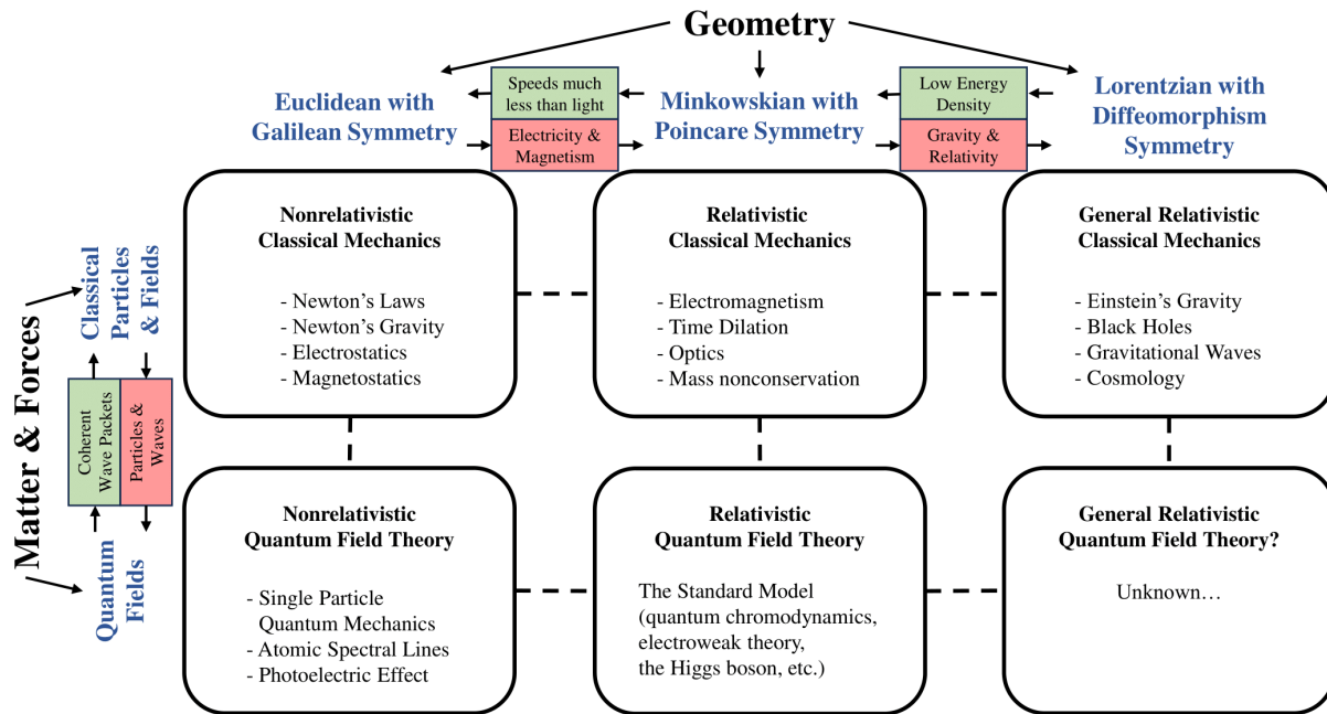
Figure 1: The map of the regimes of physical theories together with just some of the successes of each theory.
