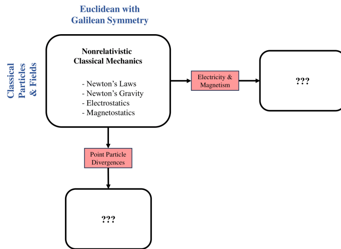
Figure 3.1: Our perspective on physics as of the end of this chapter. We have many successes and two major problems. Those two problems will be our guides for what to try next.
