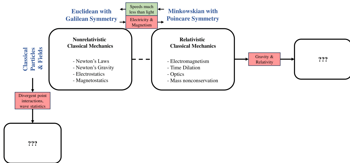
Figure 5.2: Our perspective on physics as of the end of this chapter. We have yet to work out a relativistically consistent theory of gravity which allows for mass nonconservation. We have found that point particles have divergent interactions once relativity is accounted for and that classical fields have divergent thermodynamic properties once statistical mechanics is accounted for. There is a fundamental tension between classical field theory and statistical mechanics.
