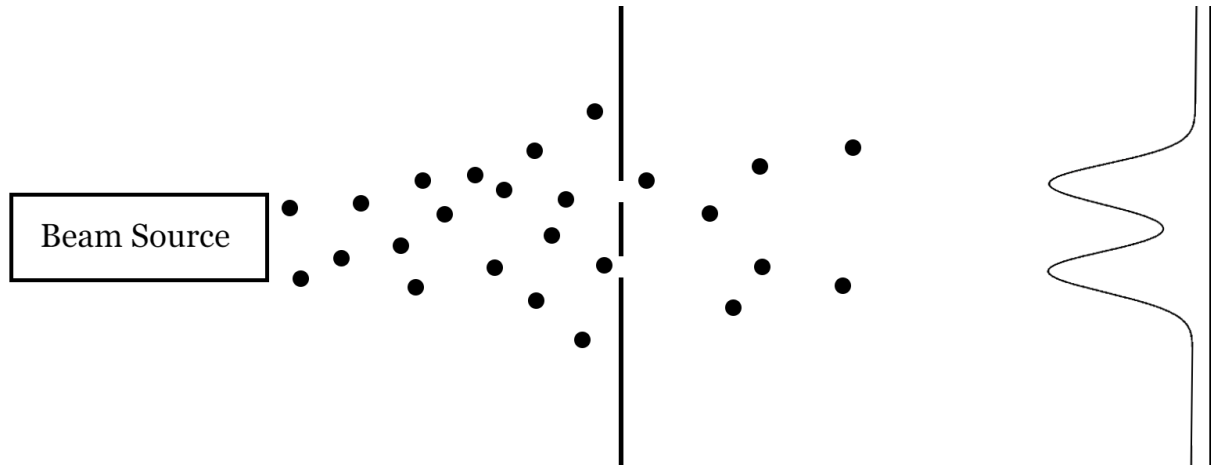
Figure 4.1: The point particle prediction for the intensity of incident particles through a double-slit apparatus. The plot given on the right hand screen is a graph of the predicted intensity versus position on the screen.
