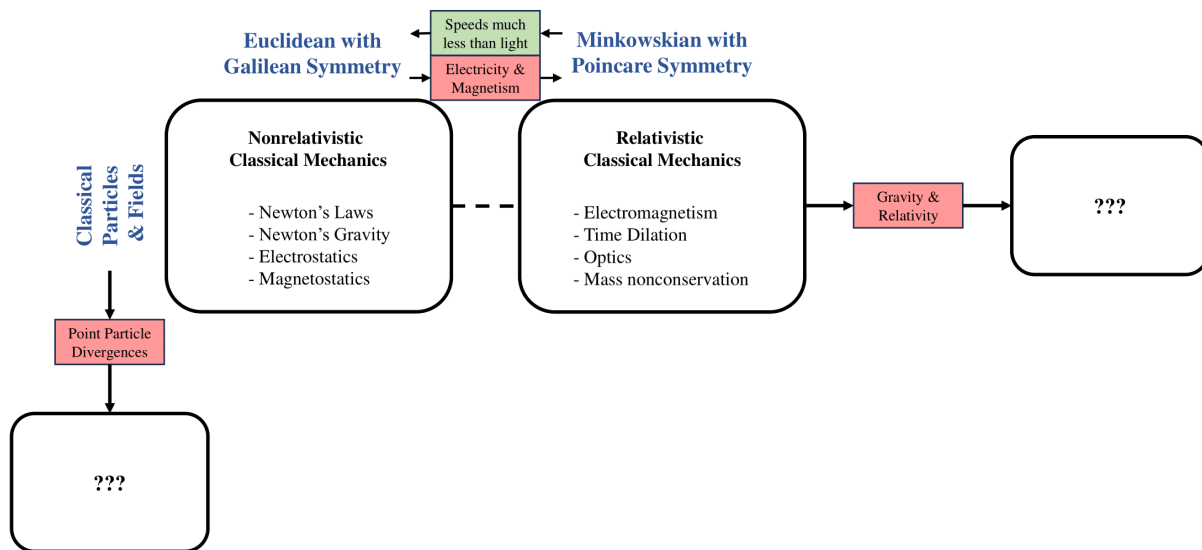
Figure 4.3: Our perspective on physics as of the end of this chapter. Lorentz boost symmetry was able to solve the problem of electromagnetic coexistence but did nothing to affect the problem of point particle divergences. As well, we found there is some more work to be done to make gravity consistent with this new boost symmetry.
