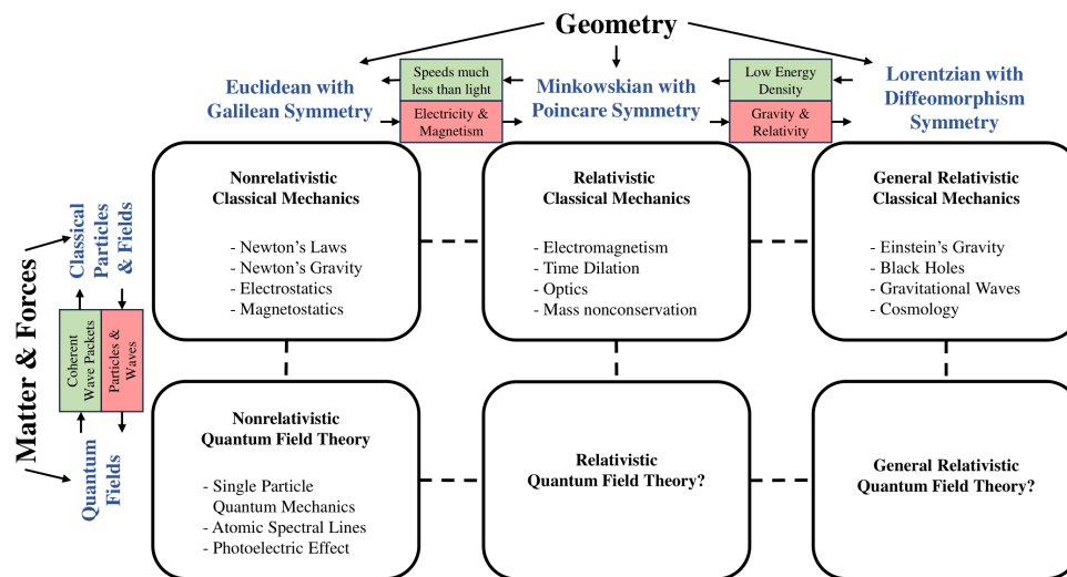
Figure 8.1: Our perspective on physics as of the end of this chapter. Replacing our point particle theory of matter with a wave theory has completely solved the problem of point particle divergences. However, so far only did so using Galilean symmetry and naturally must next work on combining Lorentz symmetry with our wave theory of matter. As well, we found that our wave theory of matter was not quite right for the statistics of multiple particles and that quantum field theory, which we haven't yet studied, is its necessary generalization to get these statistics right.
