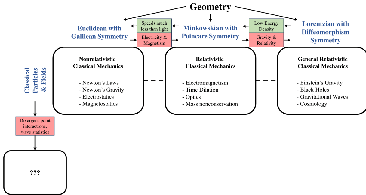
Figure 7.1: Our perspective on physics as of the end of this volume. Lorentz boost symmetry was able to solve the problem of electromagnetic coexistence but did nothing to affect the problem of point particle divergences. Diffeomorphism symmetry was able to provide for a relativistically consistent theory of gravity. However, we remain without a valid model of matter superior to point particles even though we know that point particles do not have mathematically well-defined interactions with gravity or electromagnetism. The statistical properties of classical field theory are at odds with experiment. With our knowledge so far, we cannot answer the question why does hot metal glow, because we can't even explain how metal can be hot.
