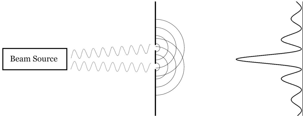
Figure 4.2: The wave theory prediction for the intensity of incident waves through a double-slit apparatus. The plot given on the right hand screen is a graph of the predicted intensity versus position on the screen.
